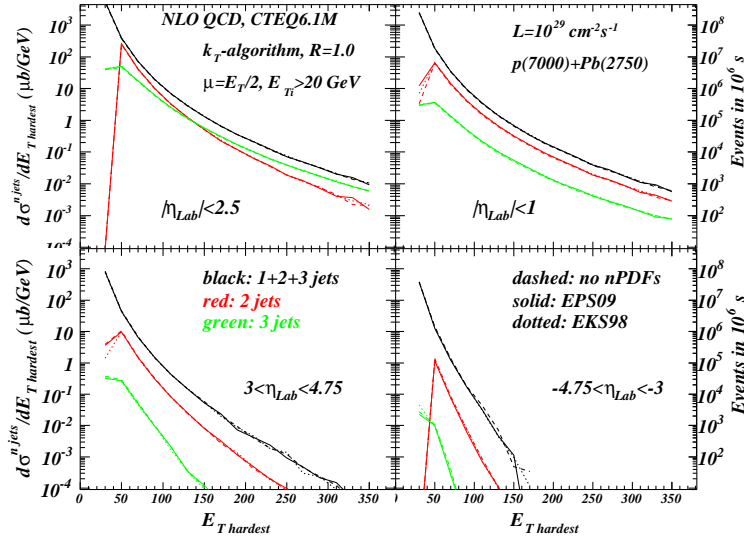
Fig. 2: 1-, 2- and 3-jet cross section as a function of the E_T of the hardest jet within the acceptance. Different pseudorapidity windows (in the laboratory frame) computed for minimum bias p+Pb collisions at the LHC (2.75+7 TeV per nucleon) are considered. Dashed lines are the results without nuclear modification to the PDFs; solid lines are the results with EPS09 [25]; dotted lines are results with EKS98 nuclear corrections [39, 40] to nucleon parton densities. Also shown is the scale for corresponding yields for a luminosity \mathcal{L} = 10^{29} \text{ cm}^{-2}\text{s}^{-1} in one month of running.
