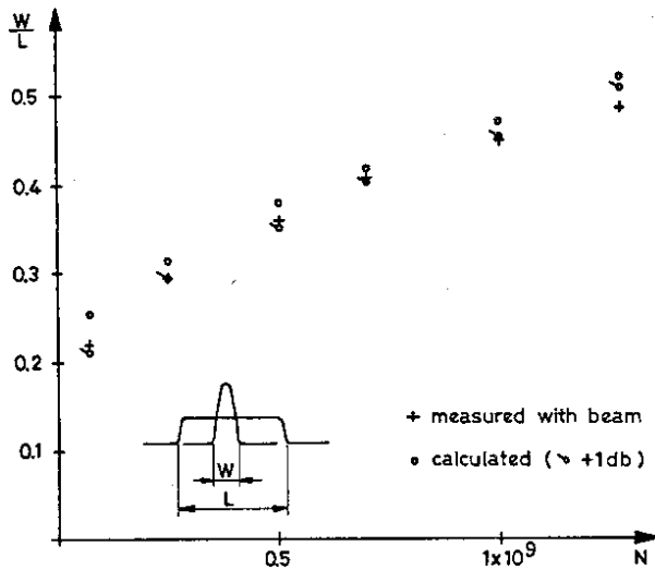
Fig. 14. Reduction of full width in \Delta p/p .
