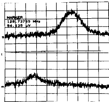
Fig. 20. Longitudinal Schottky signal from \sim 240 \bar{p} .
