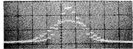
Fig. 19. Horizontal beam profile before and after cooling, as seen by a monitor based on beam-induced ionization electrons from the residual gas.
