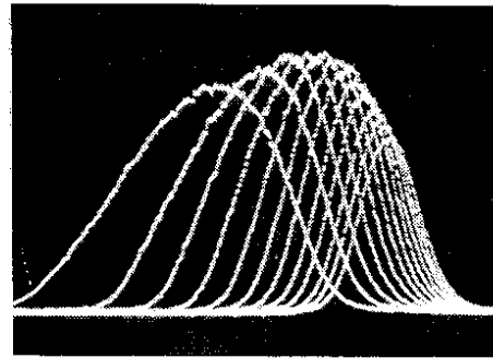
Fig. 6. Longitudinal Schottky scans at the 18th harmonic, taken at 1 min intervals. The scans are the result of spectrum analysis of longitudinal statistical beam structure. The vertical axis is \propto \sqrt{dN/df} , the horizontal is frequency.
