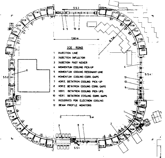
Fig. 3. General floor layout.
