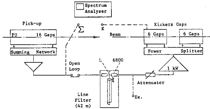
Fig. 4. General layout of \Delta p/p cooling system.
