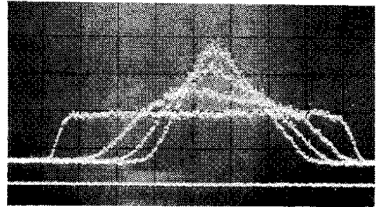
Fig. 7. 8 \cdot 10^7 p , 10 s between scans, factor 4.75 in peak density in 30 s, initial e-folding time is 15 s, average value 20 s. Cent. frequency 60 MHz, 20 kHz/cm, total initial width \Delta p/p = 3.5 \cdot 10^{-3} . The vertical axis is proportional to \sqrt{\psi} .
