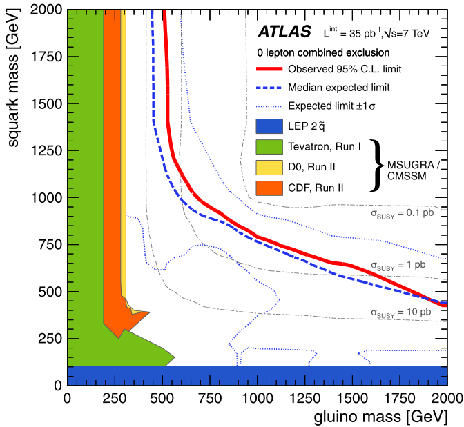
Fig. 2. 95% C.L. exclusion limits in the (m_{\tilde{g}}, m_{\tilde{q}}) plane together with existing limits [5–9] and contours showing the total supersymmetric cross section, for the simplified squark–gluino model with massless \tilde{\chi}_1^0 . Comparison with existing limits is illustrative only as some are derived in the context of MSUGRA/CMSSM or may not assume m_{\tilde{\chi}_1^0} = 0 .
