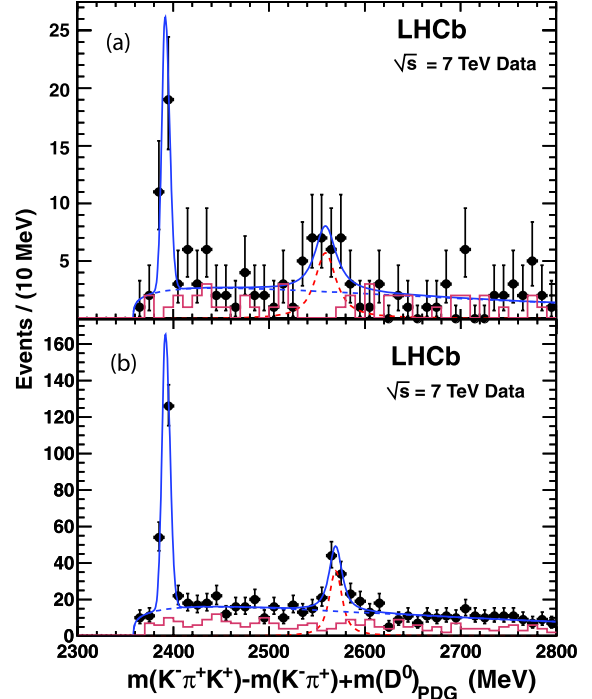
Fig. 2. The mass difference m(K^-\pi^+K^+) - m(K^-\pi^+) added to the known D^0 mass for events with K^-\pi^+ invariant masses within \pm 20 MeV of the D^0 mass (black points) in semileptonic decays. The histogram shows wrong-sign events with an additional K^- instead of a K^+ . The curves are described in the text. (a) For the 3 \text{ pb}^{-1} data sample and (b) for the 20 \text{ pb}^{-1} sample.
