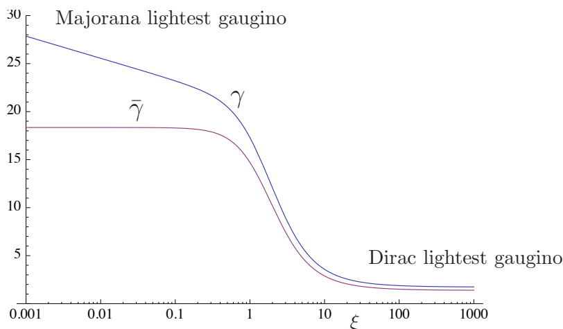
Figure 1. The ratio \gamma \equiv 8\pi^2\Pi/M_\lambda^2 where the scalar mass-squareds are m_i^2 = 4g^2C(R_i)\Pi , in a slice of \text{AdS}_5 with supersymmetry breaking on the IR brane (taken from ref. [56]). The upper line is the zero momentum value, the lower line is the value at the messenger scale. The lightest gaugino mode varies continuously from Majorana to pure Dirac as the relative supersymmetry breaking on the IR brane, \xi , increases. Note from the figure that the Majorana mass term is logarithmically renormalized (hence the difference between the two lines) while the (finite) Dirac mass term is not.
