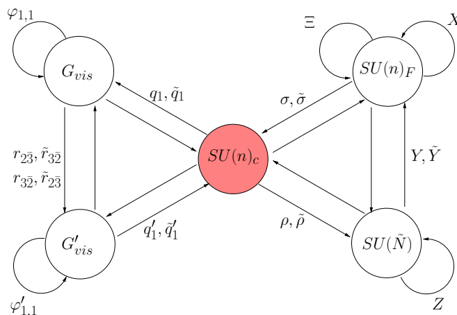
Figure 7. The magnetic Seiberg dual of the quiver in figure 6. Supersymmetry is broken by the rank-condition with the SU(\tilde{N}) node providing the F -term breaking: F_Z \neq 0 .
