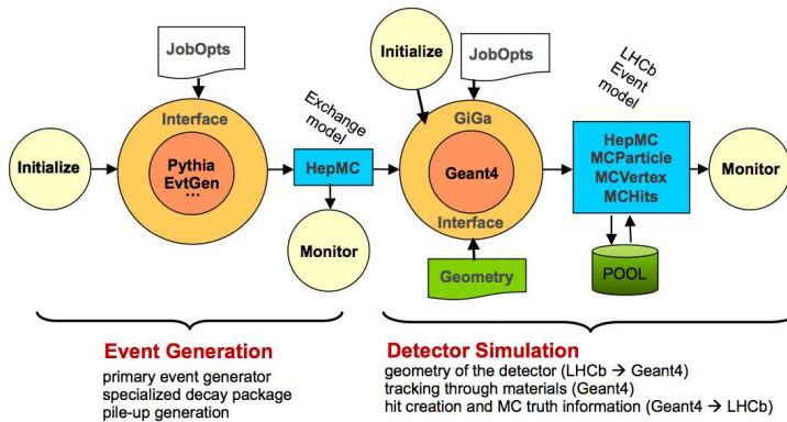
Figure 1. Structure of the Gauss software.
