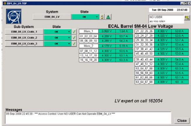
Figure 5: SM LV panel
