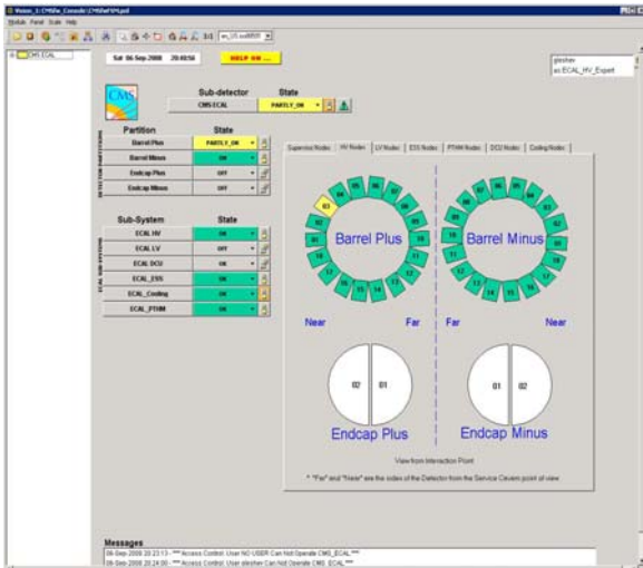
Figure 2: ECAL Supervisor main panel
