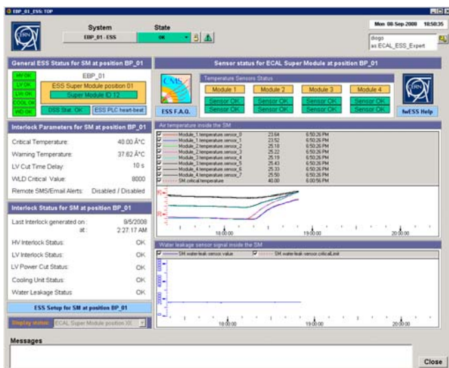
Figure 9: ESS SM panel
