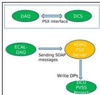
Figure 6: Software connection between DAQ and DCS
