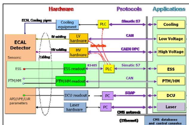
Figure 1: ECAL DCS layout
