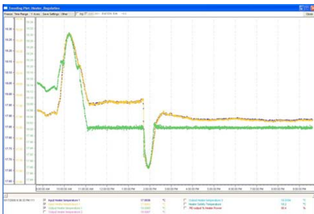
Figure 3: Cooling regulation (time x input and output temperatures)
