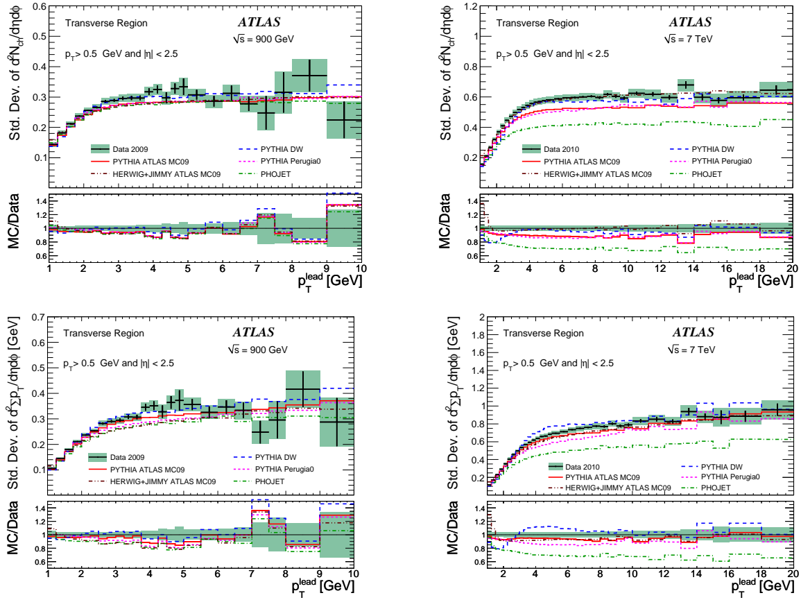
FIG. 5. ATLAS data at 900 GeV (left) and at 7 TeV (right) corrected back to the particle level, showing the standard deviation of the density of the charged particles \langle d^2N_{ch}/d\eta d\phi \rangle (top row) and the standard deviation of the scalar \sum p_T density of charged particles \langle d^2\sum p_T/d\eta d\phi \rangle (bottom row) with p_T > 0.5 GeV and |\eta| < 2.5 , as a function of p_T^{\text{lead}} , for the transverse region defined by the leading charged particle and compared with PYTHIA ATLAS MC09, DW and Perugia0 tunes, HERWIG+JIMMY ATLAS MC09 tune, and PHOJET predictions. The error bars show the statistical uncertainty while the shaded area shows the combined statistical and systematic uncertainty.
