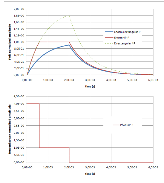
Figure 2: Pulse shape of cavity field and necessary klystron power pulse in tests without beam.
