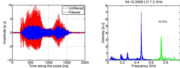
Figure 6: (a) An example of the time domain output of the RF pickup detector (red), with the 33 GHz beam component filtered (blue). (b) The time averaged FFT of the red output signal shown in 6 (a).
