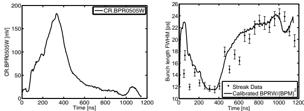
Figure 5: (a) Analog single shot response from BPRW in the combiner ring. (b) Bunch Length measurement comparing calibrated BPRW and the Streak Camera.
