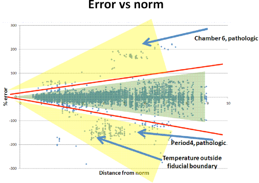
Figure 9: Distribution of error as a function of the \|\mathbf{x}\| norm for all runs, six chambers and both training and prediction.
