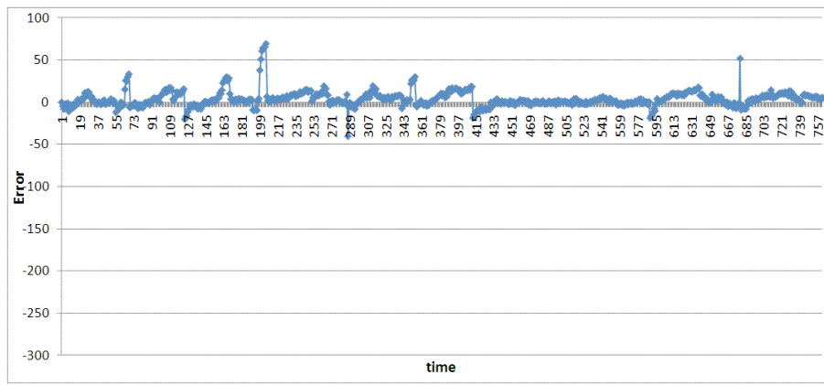
Figure 16: Period 2 training, prediction on periods 3 and 1, fiducial selection
