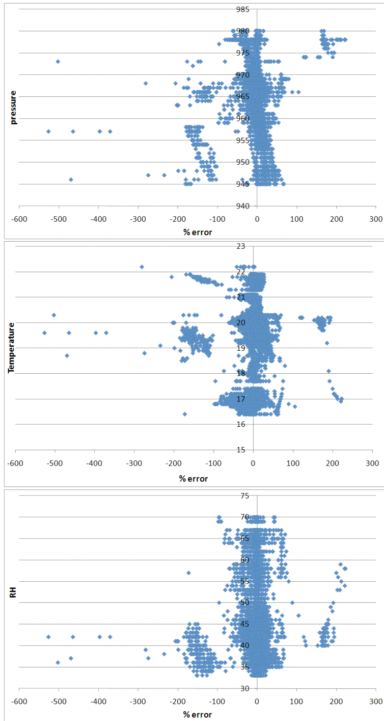
Figure 8: (Top) pressure (center) temperature (bottom) humidity versus error \frac{\Delta Q}{Q}
