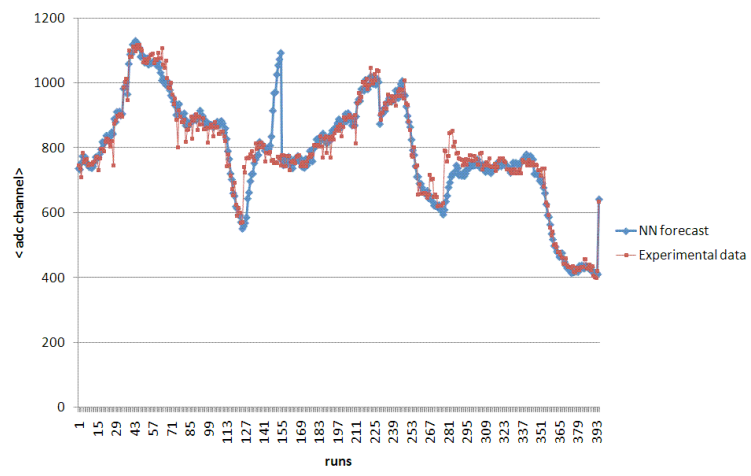
Figure 4: Gap 8 trained on period 1 - prevision on period 1
