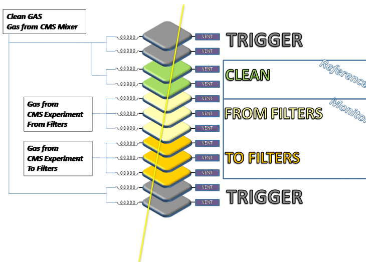
Figure 2: Layout of GGM experimental setup
