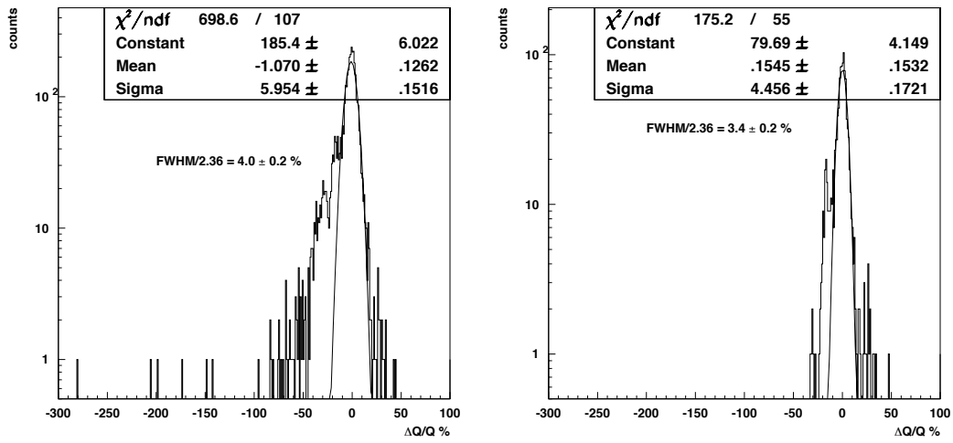
Figure 14: Period 1 training, prediction on periods 2 and 3, (left) no cuts, (right) fiducial cut, gaussian fit superimposed.
