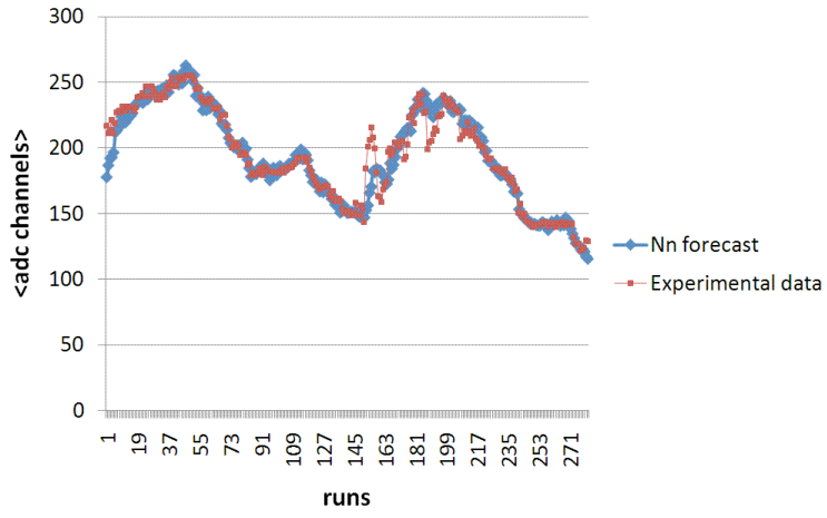
Figure 3: Gap 7 trained on 3 - prevision on period 3
