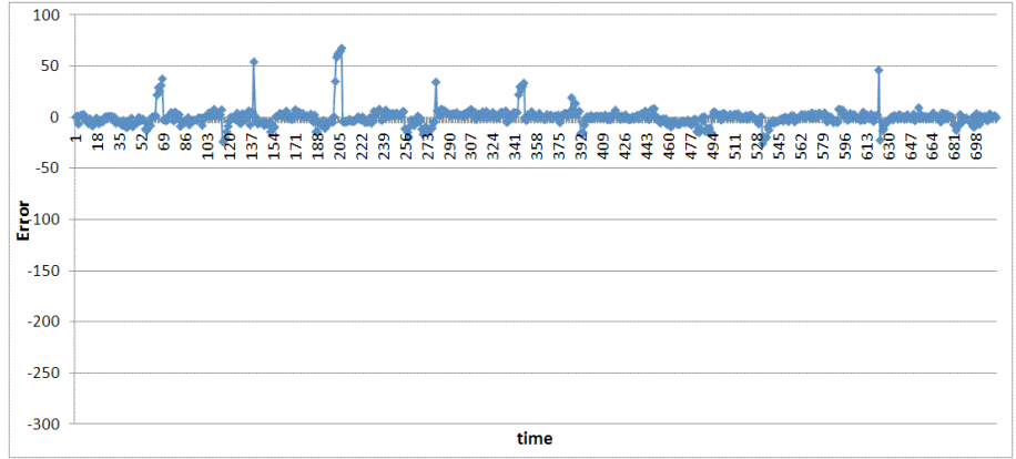
Figure 19: Period 3 training, prediction on periods 1 and 2, fiducial selection.
