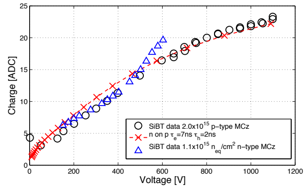
Figure 4: Comparison on n-type and p-type MCz charge collection efficiency. The dashed line represents a transport model prediction that has been tuned to fit the p-type data. A non-clustering approach was used for the the p-type data.
