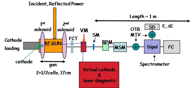
Figure 1. Photo injector layout: symbols explanation is given in the text.
