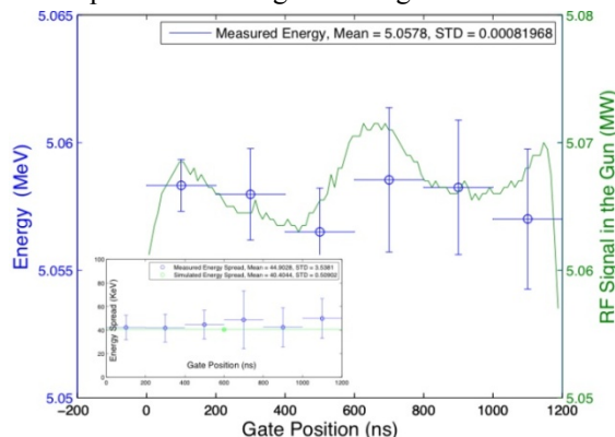
Figure 5: Energy and the energy spread along the pulse.
