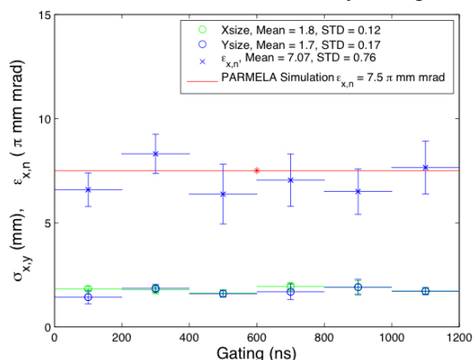
Figure 4: Beam sizes and the emittance along the pulse.
