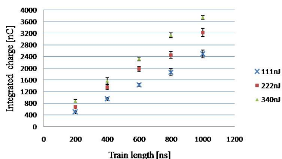
Figure 2: Integrated charge as function of train lengths for three different laser pulse energies: 111, 222 and 340 nJ. Laser transverse size \sigma \sim 0.3 mm.
