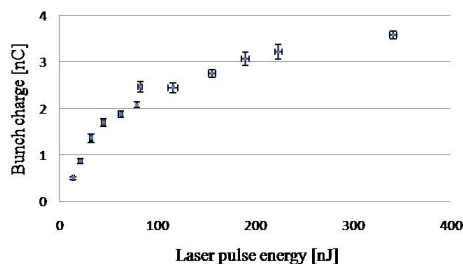
Figure 3: Electron bunch charge as a function of the laser pulse energy for 200ns train of laser pulses. Laser transverse size: \sigma \sim 0.3 mm.
