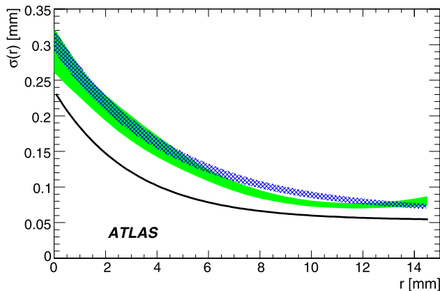
Fig. 12 Drift tube resolution as a function of the radius. The green shaded (RPC correction method) and the blue hatched ( Gt_0 -refit method) bands represent the resolution function measured with cosmic rays with the two different methods described in the text. The solid line represents the resolution measured with a high momentum muon beam [5]
