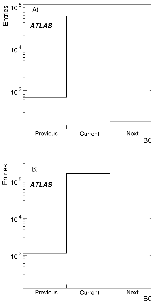
Fig. 6 (A): TGC front-end and (B): sector logic buffers for BC identification. Three BC crossing, previous, current and next are readout
