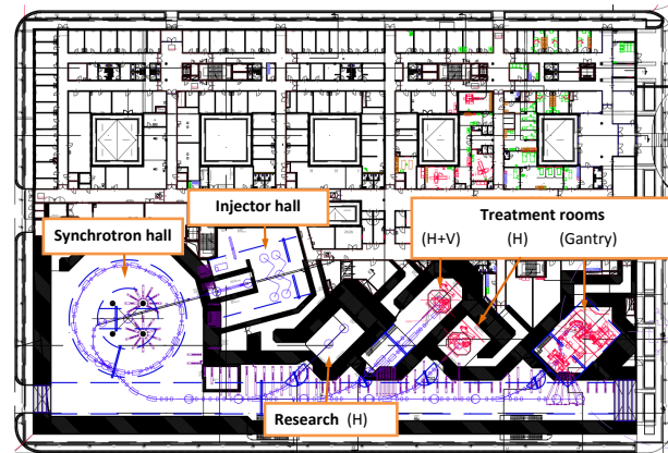
Figure 1: Ground floor of the MedAustron facility. Upper part: offices and medical rooms. Lower part: Synchrotron hall, injector hall and irradiation rooms. "H" denotes horizontal beam line and "V" vertical beam line.
