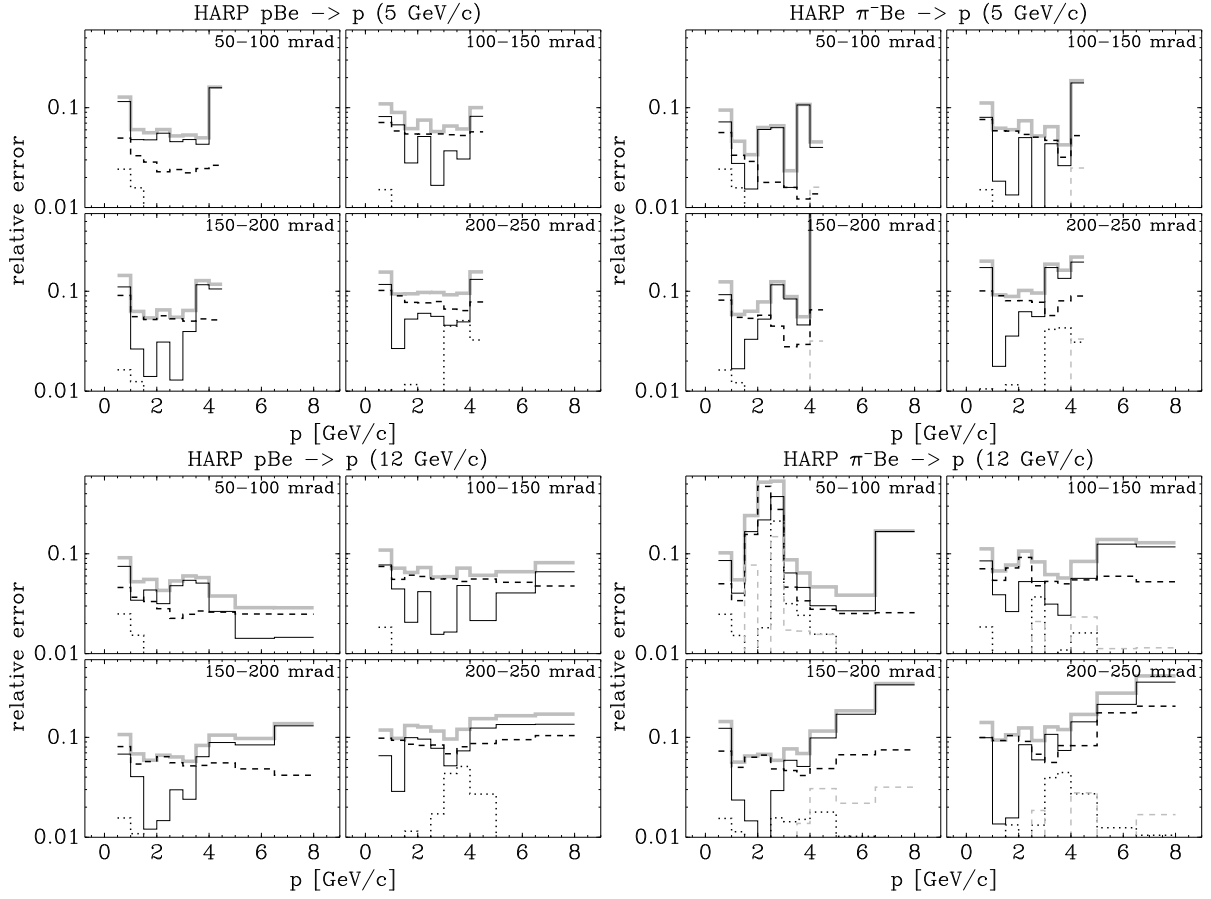
FIG. 2: Total systematic error (grey solid line) and main components for a typical (Be) target with incident p and \pi^- beams at 5 and 12 \text{GeV}/c black short-dashed line for absorption+tertiaries interactions, black dotted line for track efficiency and target pointing efficiency, black dot-dashed line for \pi^0 subtraction, black solid line for momentum scale+resolution and angle scale, grey short-dashed line for PID.
