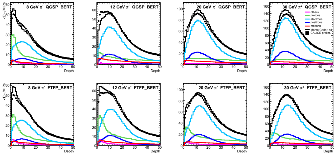
Figure 14: Longitudinal energy profiles for data (shown as points) compared with simulations using two physics lists, QGSP_BERT and FTFP_BERT, at four typical energies. The breakdown of the Monte Carlo into the energy deposited by different particle categories is also indicated.
