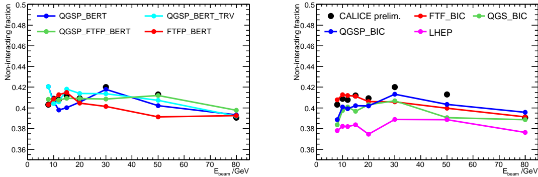
Figure 5: Mean fraction of non-interacting pions (energy < 100 MIPs) in the ECAL, plotted as a function of beam energy. The data are compared with the predictions of simulations using different GEANT4 physics lists.
