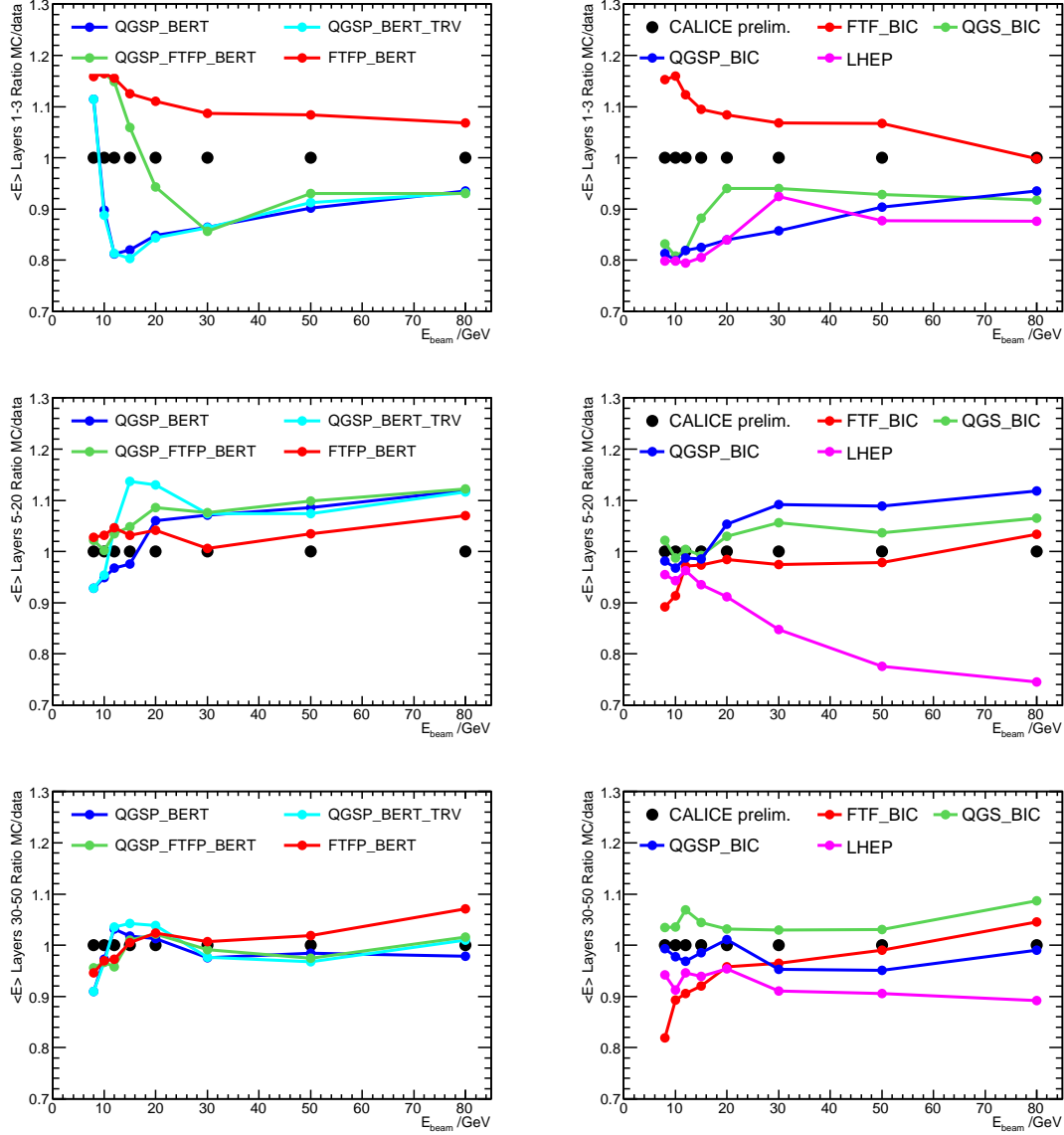
Figure 15: Ratio of simulation to data for three different regions of the longitudinal energy profile: (top pair of plots) layers 1-3, dominated by nuclear breakup; (centre pair) layers 5-20, dominated by electromagnetic showers; and (bottom pair) layers 30-50, dominated by penetrating hadrons.
