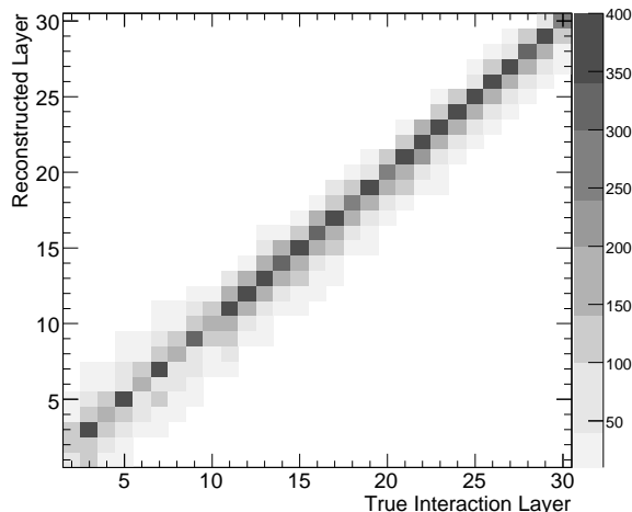
Figure 11: Comparison between reconstruction and truth for the layer identified as the interaction layer by the algorithm described in the text. The distributions are normalised to the same numbers of events. This case corresponds to a 20 GeV \pi^- beam, using the QGSP_BERT physics list in the case of the simulation. Bins containing fewer than 10 events have been suppressed for the sake of clarity.
