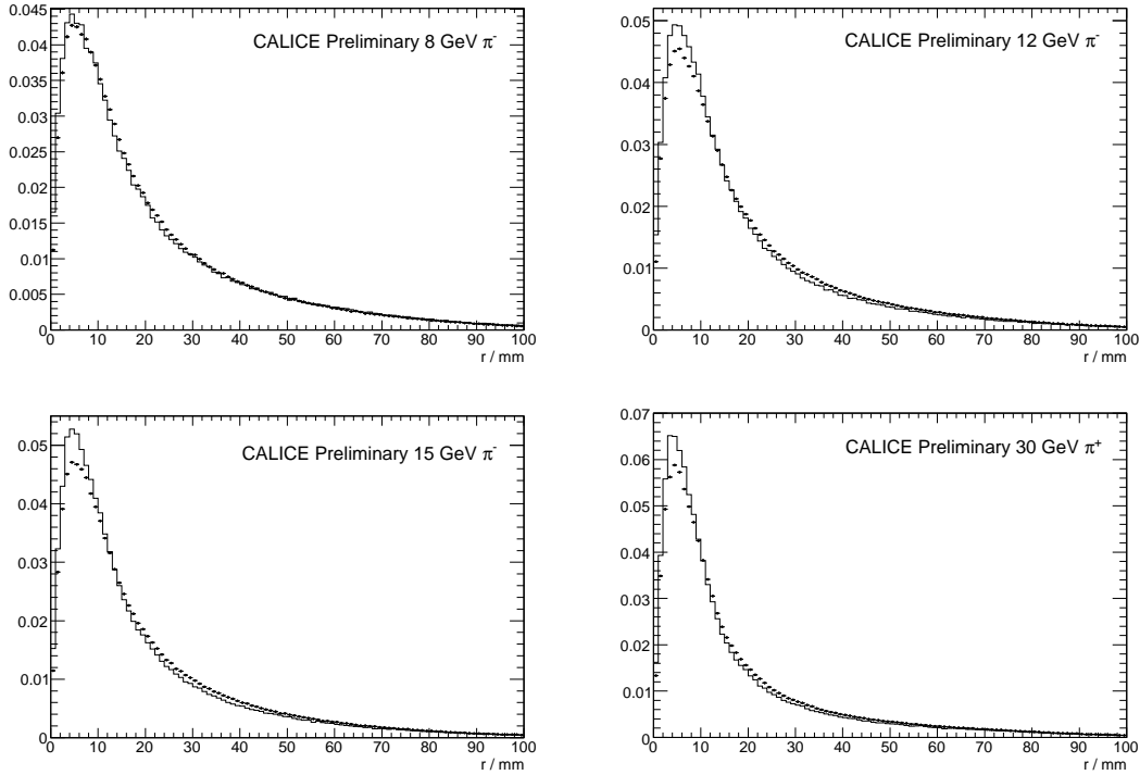
Figure 8: Radial distribution of hits (energy weighted) for data at four typical energies (points with errors) compared with Monte Carlo (solid line) using the QGSP_BERT physics list. The distributions are normalised to unity.
