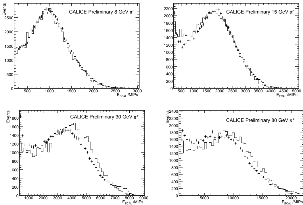
Figure 6: Distributions of total energy recorded in the ECAL at 8, 15, 30 and 80 GeV (points with error bars), compared with Monte Carlo predictions using the QGSP_BERT physics list (solid lines). The distributions are normalised to the same numbers of selected events (including the non-interacting peak).
