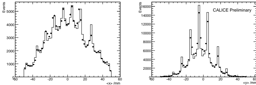
Figure 2: Example of the beam profiles in x and y observed with a 20\text{ GeV } \pi^- beam. Data (points with error bars) are compared with the tuned simulation (solid histogram). The distributions are normalised to the same numbers of events.
