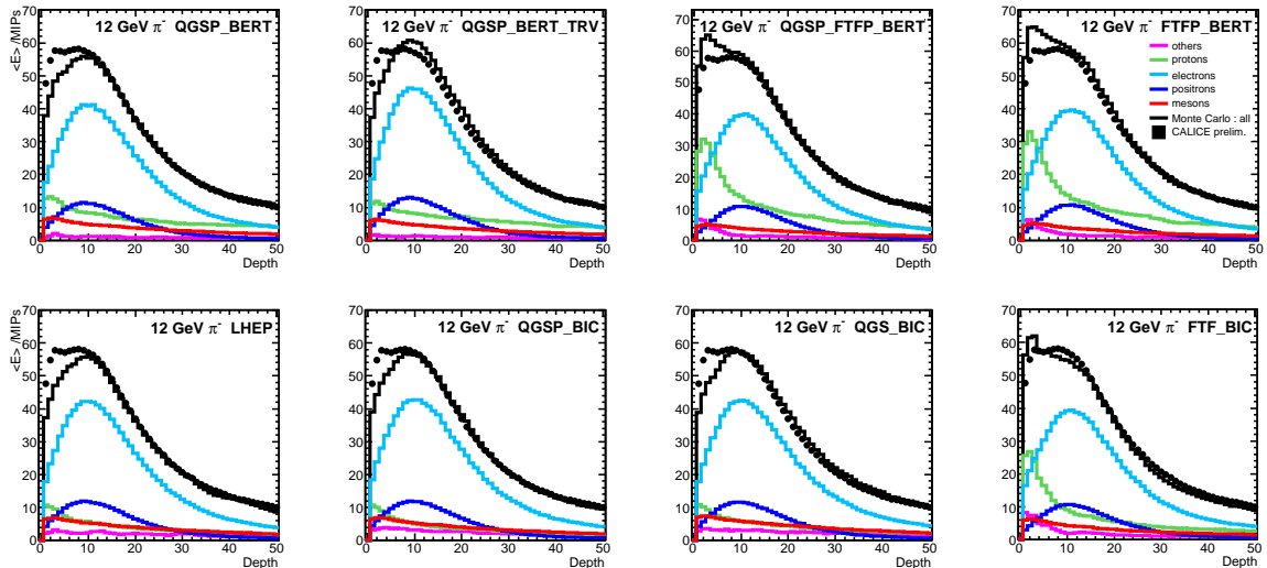
Figure 13: Longitudinal energy profiles for 12 GeV \pi^- data (shown as points), compared with simulations using different physics lists. The mean energy in MIPs is plotted against the depth after the initial interaction, in units of effective 1.4 mm tungsten layers. The total depth shown corresponds to \sim 20 X_0 or 0.8 \lambda_{\text{int.}} . The breakdown of the Monte Carlo into the energy deposited by different particle categories is also indicated.
