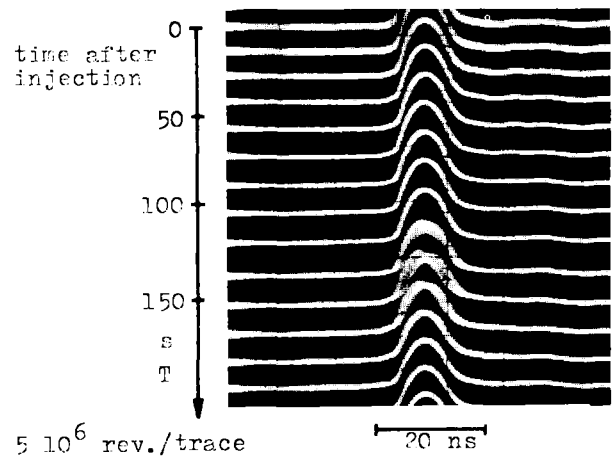
Fig. 7. A bunch stabilized with the higher harmonic cavity.
