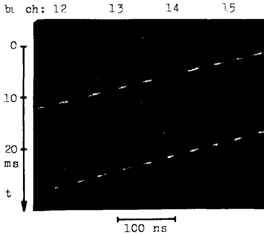
Fig. 3. Coupled bunch oscillations. Bunches with the same phase are connected by the oblique, dashed line.
