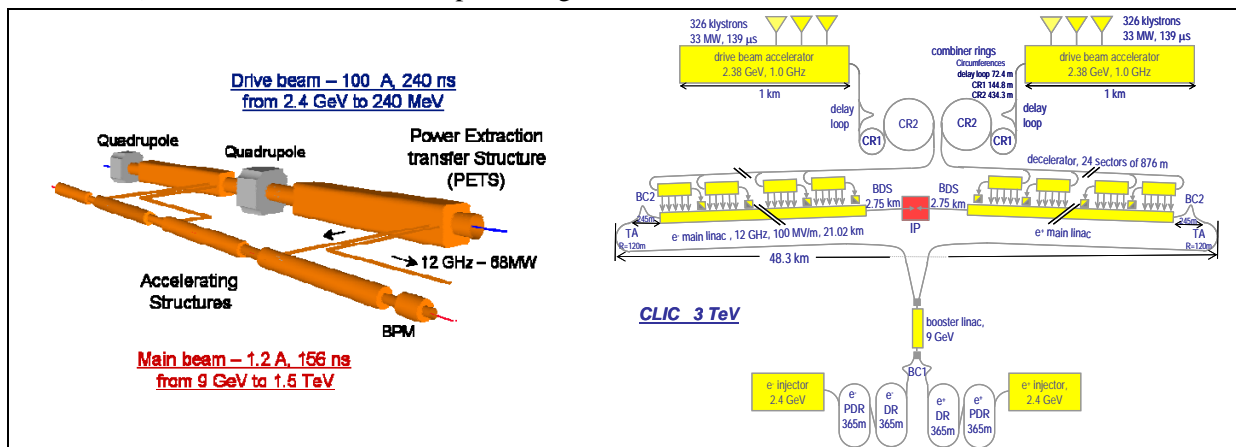
Fig. 4: CLIC two-beam scheme. The right picture shows the complete complex with the Drive Beam generation complex on top and the Main Beam generation at the bottom
