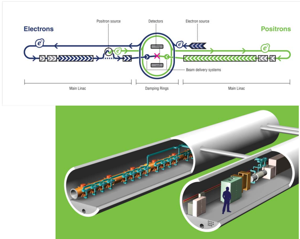
Fig. 3.: ILC base-line design (top) and at the bottom the two-tunnel layout with the main accelerator tunnel on the left, the klystron and service tunnel on the right.
