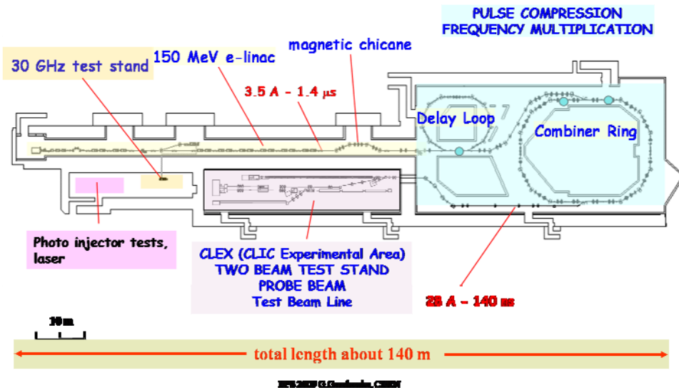
Fig. 5: CTF3 layout
