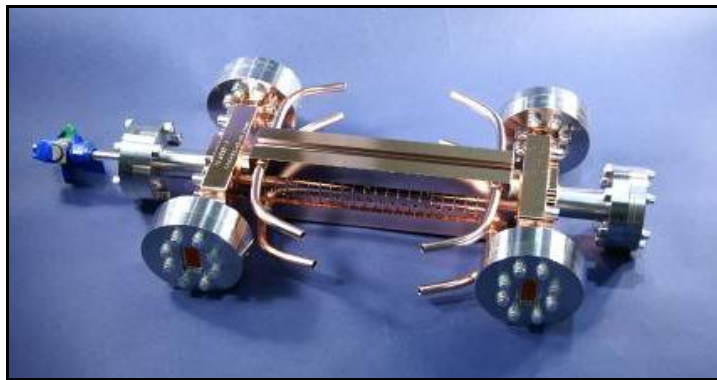
Fig. 2: CLIC accelerating structure
