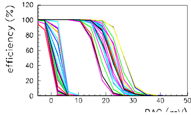
Figure 20: 36 channels S-curves
