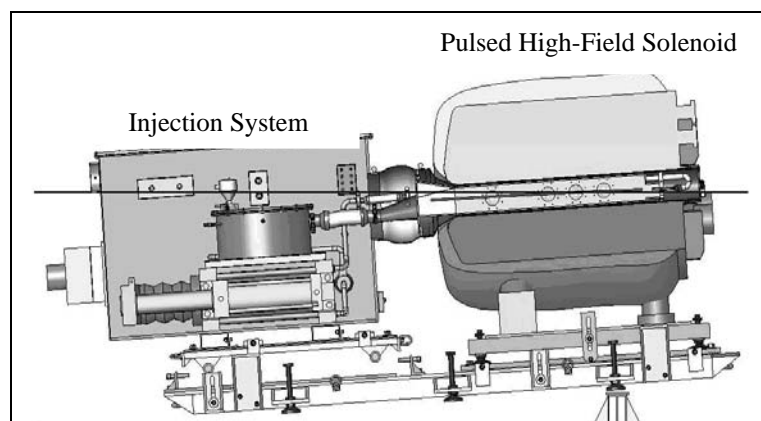
FIGURE 1. The pulsed high field magnet mated with the Hg injection system. The Hg jet intercepts the proton beam within the confines of the magnet.
