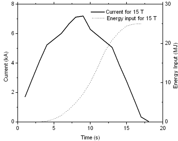
FIGURE 2. A magnet pulse of 15 T by ramping the current up and down. During the current plateau the beam intercepted the Hg jet. Energy deposition reached a maximum of 25 MJ.
