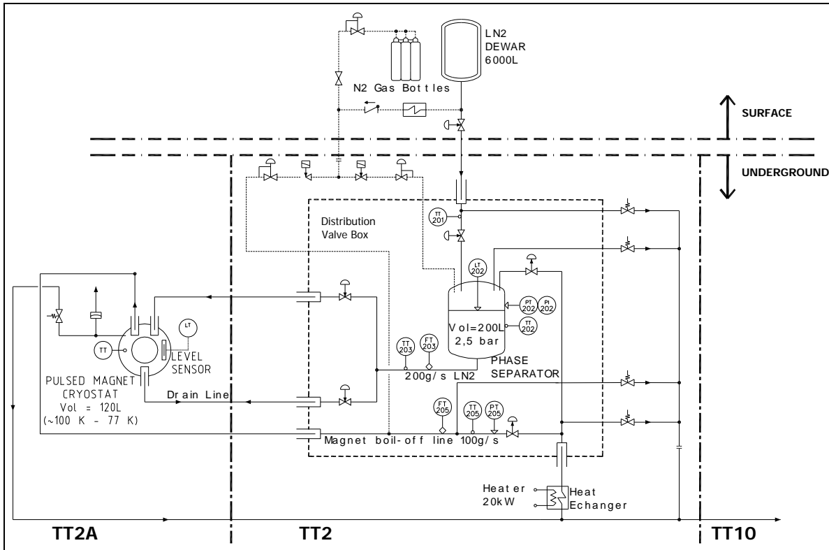
FIGURE 4. MERIT flow scheme.
