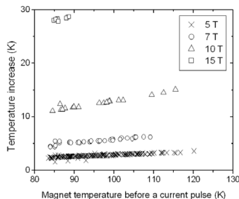
FIGURE 6. Magnet temperature increase for various current pulses as a function of the initial magnet temperature.
