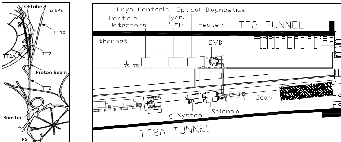
FIGURE 5. (a) CERN PS extraction tunnel complex. (b) Plan of the MERIT layout in the TT2 and TT2A tunnels.
