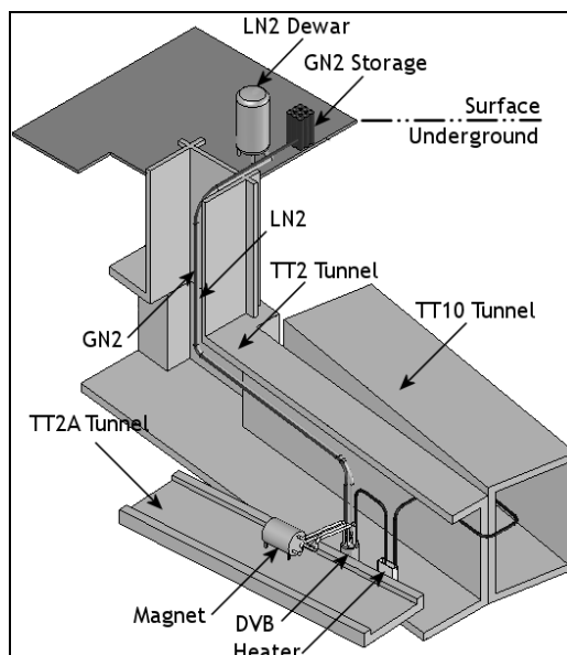
FIGURE 3. Layout of the cryogenic system.
