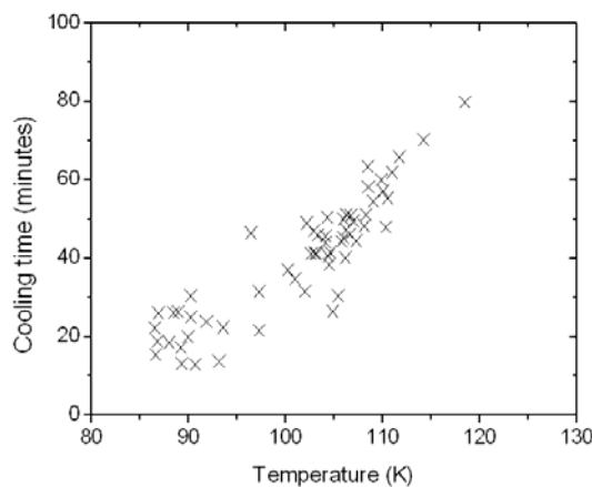
FIGURE 8. Cooling cycle time as a function of the magnet temperature.
