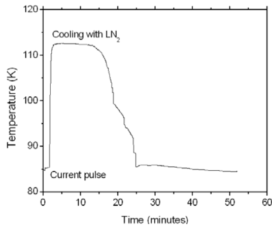
FIGURE 7. Magnet cryostat average temperature evolution for a cooling cycle after a 15 T pulse.
