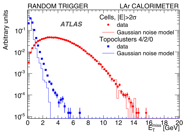
Fig. 10 E_T^{\text{miss}} distribution with LAr calorimeter cells for 135,000 randomly triggered events in June 2009. The dots (squares) show the cell-based (cluster-based) methods in the data, and the histograms show the equivalent distributions for the Gaussian noise model (see text)
