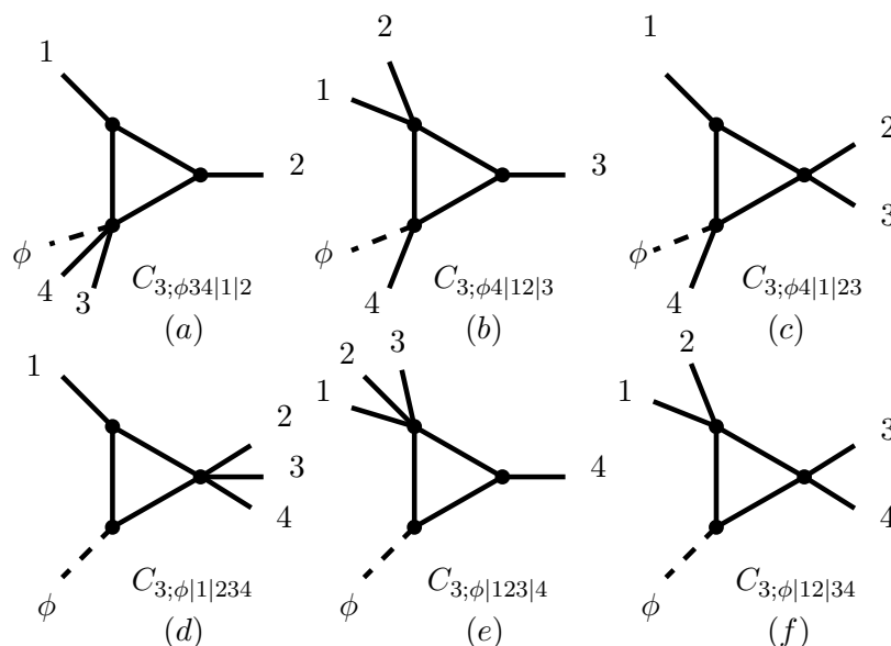
Figure 2. The various triangle integral topologies that appear for A_4^{(1)}(\phi, 1, 2, 3, 4) . From the six topologies we must also include cyclic permutations of the four gluons. (a) has one off-shell leg, (b)–(e) have two off-shell legs while in (f) all legs are off-shell.
