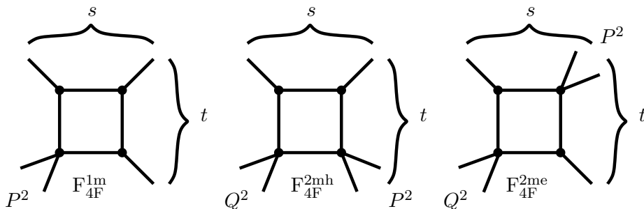
Figure 4. Conventions for labelling the three scalar box integrals appearing in the one-loop Hgggg amplitudes.
