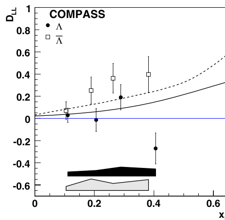
Fig. 5 The x_F dependence of the longitudinal spin transfer to \Lambda and \bar{\Lambda} . The solid line corresponds to the theoretical calculations of [2] (Model B, SU(6), CTEQ5L) for \Lambda and the dashed line is for the \bar{\Lambda} spin transfer. The shaded bands show the size of the corresponding systematic errors
