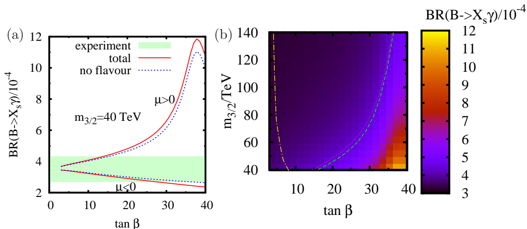
Figure 4. Constraints on the AMSB parameter space from the rare decay B \rightarrow X_s \gamma . (a) BR(B \rightarrow X_s \gamma) as a function of \tan \beta for m_{3/2} = 40 TeV and both signs of \mu . (b) BR(B \rightarrow X_s \gamma) displayed as the background colour for \mu > 0 in the \tan \beta - m_{3/2} plane. For the explanation of the various curves in both panels see the text.
