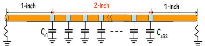
Figure 6: Equivalent schematic of simulation on signal integrity for transmission-line readout board.
