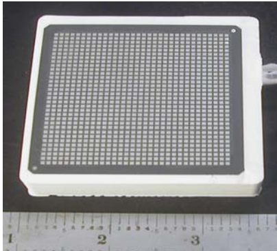
Figure 1: View of 32 x 32 anodes on the back of Burle/Photonics' tube X85011.
