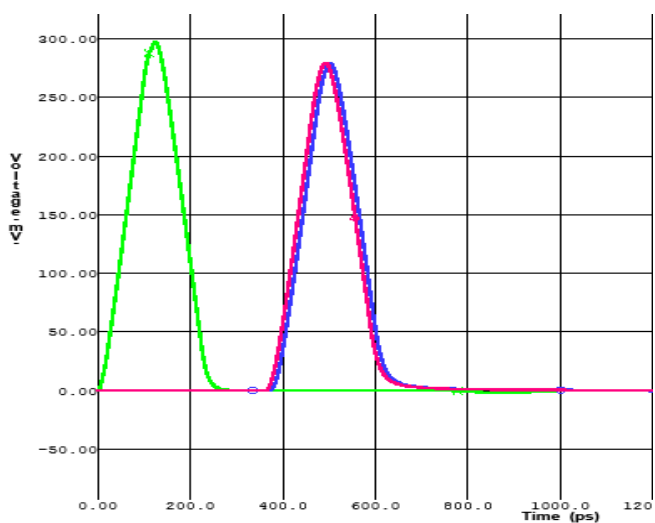
Figure 8: Simulation result of transmission-line without stub-tied anodes. The input force with 100ps rise time applied to pad #16. The green is the input force; the red is output waveform at
