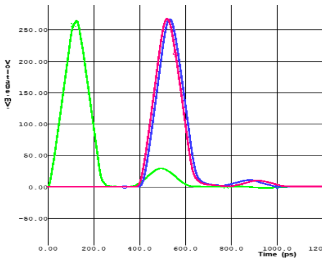
Figure 7: Simulation result of signal integrity on the transmission line with 32 stub-tied anodes. The input force with 100ps rise time is applied to pad #16. The green is the input force; the red is output waveform at the left end of the line; the blue is the output waveform at the right end of the line. The line is designed with 50-ohms and terminated at each end.
