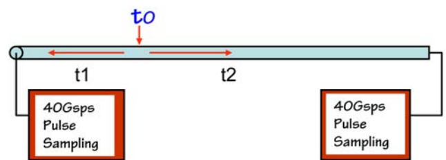
Figure 9: A diagram of transmission-line readout system using fast sampling circuits, aimed to achieve a one to few picoseconds timing resolution.
