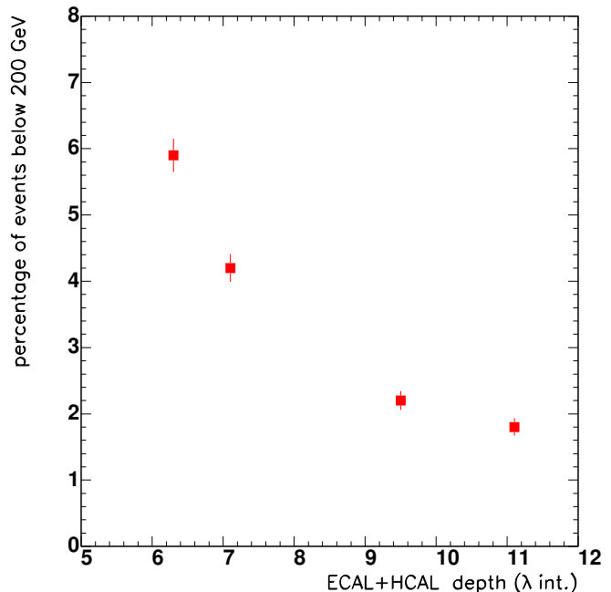
Fig. 3. Fraction of 300 GeV/c pion data with reconstructed energy less than 200 GeV (approximately 3\sigma below the mean, and corresponding to more than 100 GeV missing energy) versus total absorber depth obtained from 1996 test beam data at 3 T magnetic field. The total \lambda_{\text{int}} includes the contribution of the electromagnetic calorimeter.
