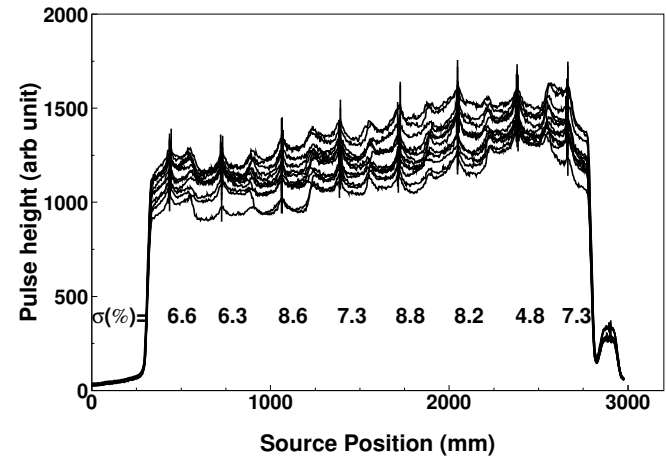
Fig. 8. Scan of a set of 12 fully assembled scintillator trays (of the 12 sectors) belonging to ring 0 layer 0 tray position 3 using the XY scanner. The lines on the figures refer to the peak positions corresponding to the centre of the tiles. The tiny peak on the right side is due to a calibration tile used in each set of measurements.
