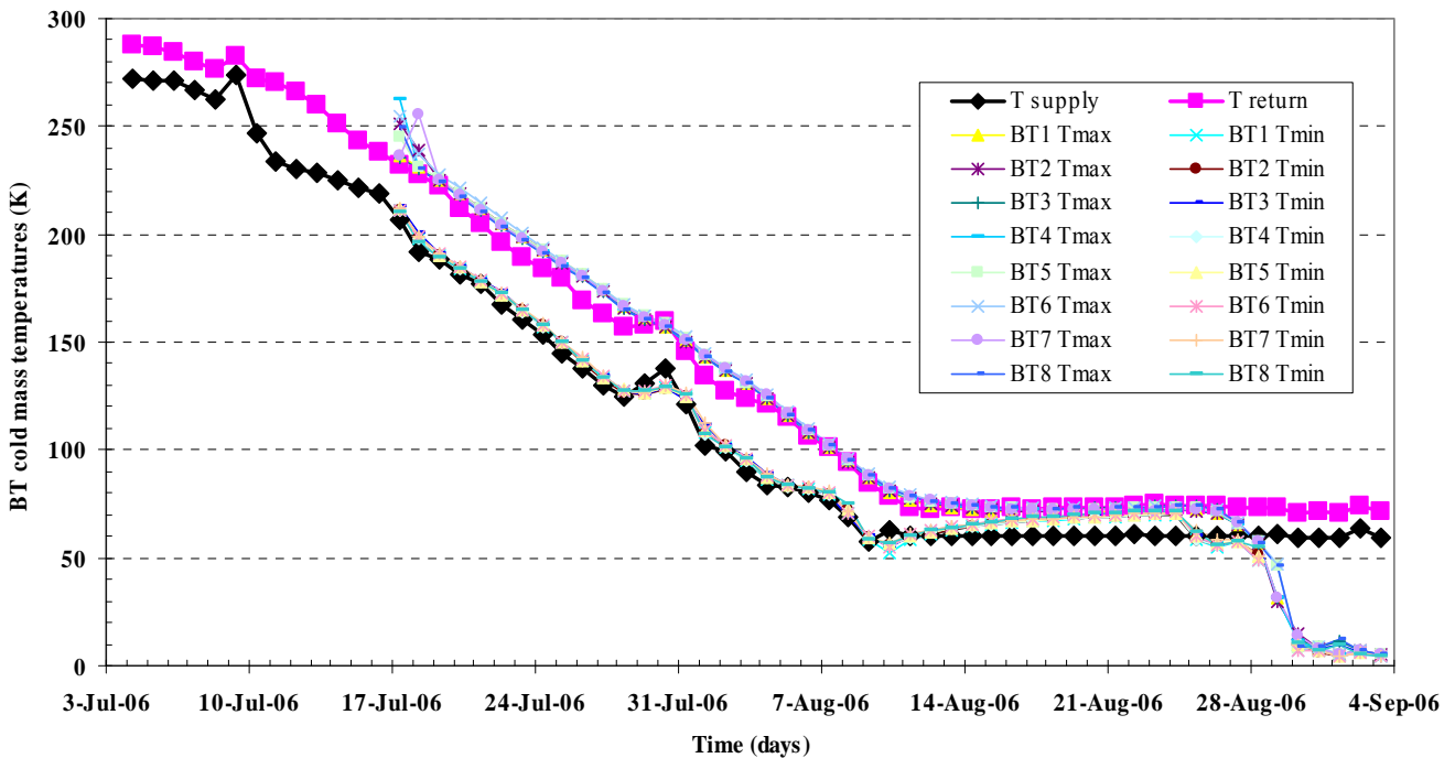
Fig. 3: Parallel cool-down of the 8 Barrel Toroid coils.
