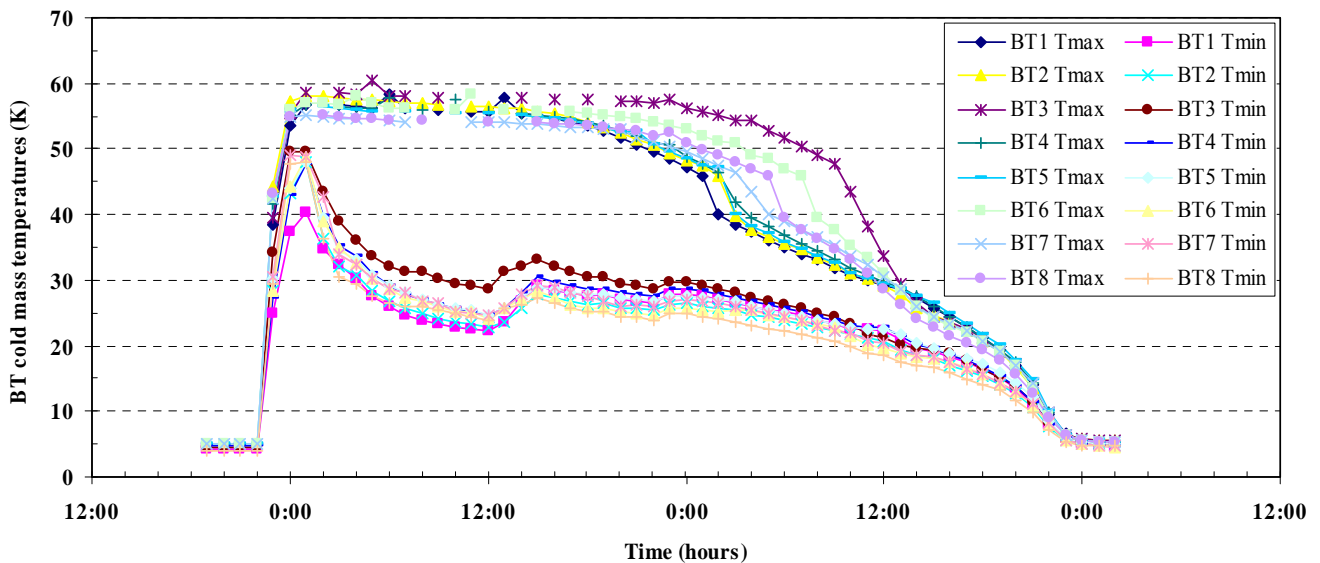
Fig. 5: Barrel Toroid recovery after a fast dump at 20.5 kA
