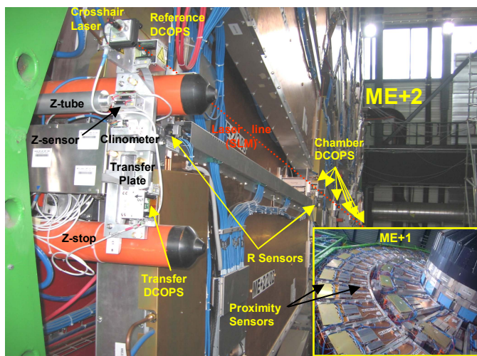
Fig. 5. Close-up of one of the three Straight Line Monitors (SLM) on the ME+2 station with crosshair laser, DCOPS, and analog sensors (R, Z, Clinometer). The inset indicates the locations of Proximity sensors on ME+1.
