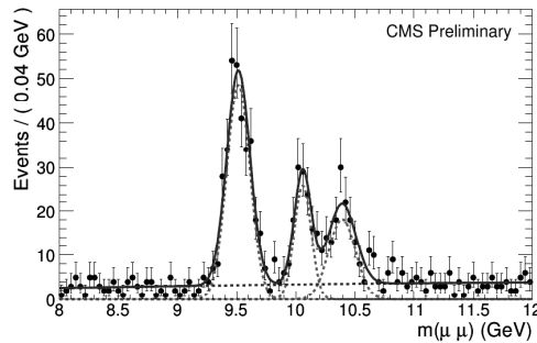
Figure 1: Dimuon invariant mass, for the selected sample, in the range 8 \leq M_{\mu^+\mu^-} \leq 12 GeV. Dashed lines are results of a fit and full line their sum. The \Upsilon(1S) , \Upsilon(2S) and \Upsilon(3S) are visible above the \gamma\gamma continuum.
