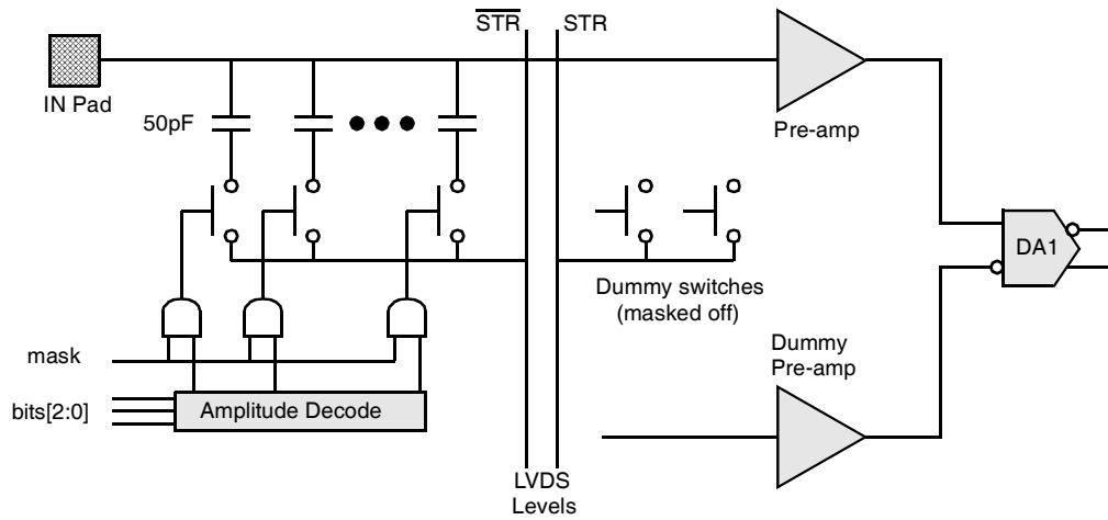
Figure 29. The MDT front-end electronics calibration system. A variable amplitude calibration pulse, labeled STR in the schematic, is introduced into selected ASD channels.
