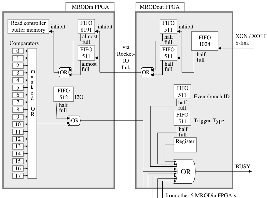
Figure 40. Busy signal generation.
