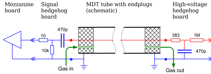
Figure 3. Main service connections to a MDT tube. At the HV side the wire is terminated with the equivalent transmission line impedance of the tube ( 383 \Omega ) to avoid reflections. All contacts (round dots) between the chamber and the hedgehog boards are gold plated to ensure a long-term connectivity.
