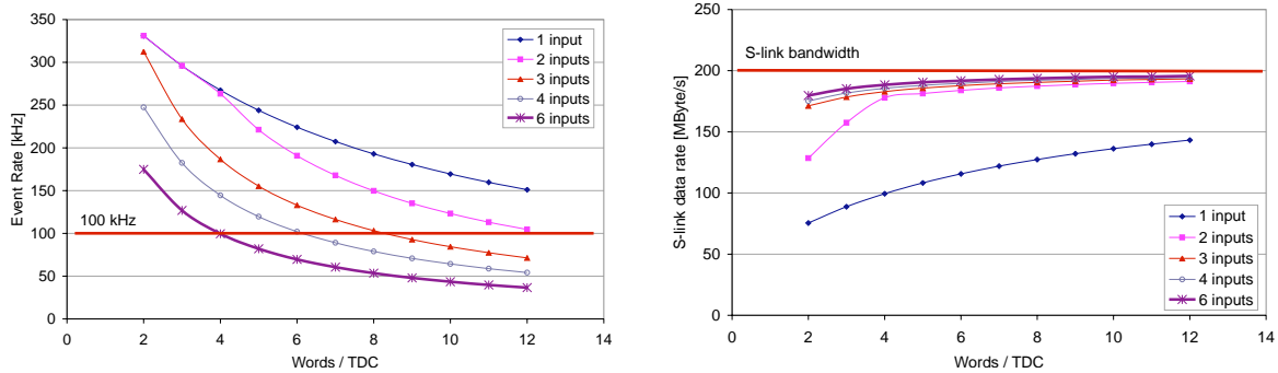
Figure 41. Maximum event rate and associated output bandwidth for the MROD as function of the number of words per TDC, with each active input receiving simulated data from 18 TDC's and for each TDC the same number of words.
