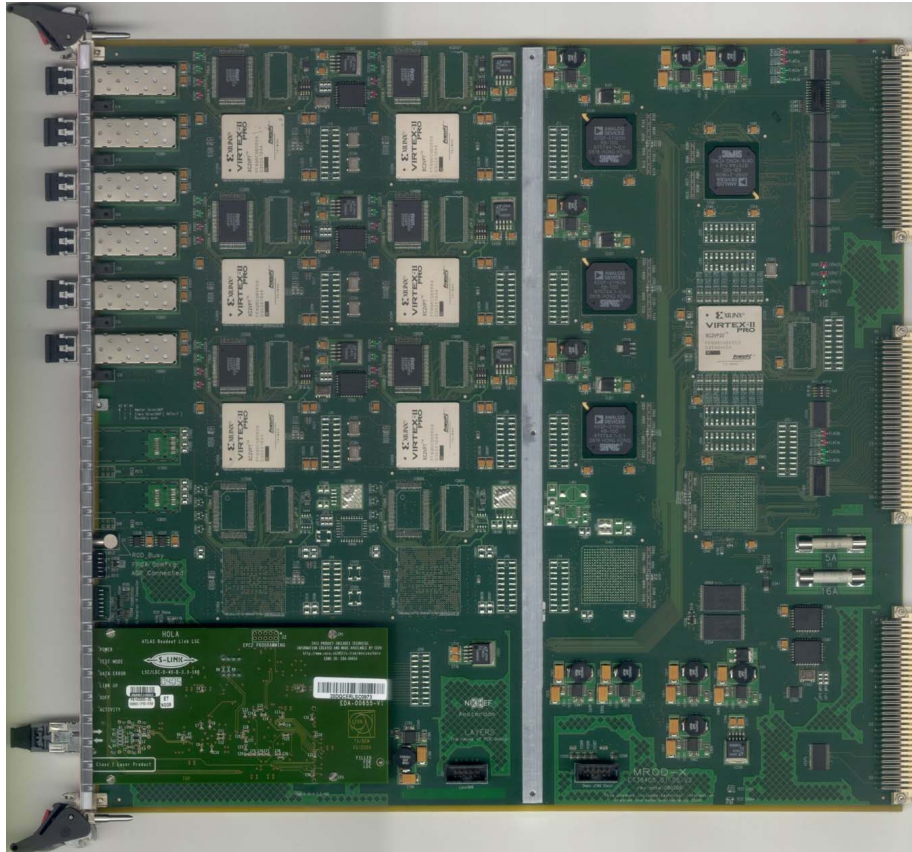
Figure 36. The MROD board. Optical fibers from up to 6 CSM's are connected at the upper left. The metallic square integrated circuits are the FPGA's, those of the MRODin sections can clearly be seen at the upper and middle left, the MRODout FPGA is at the middle right. The large black square integrated circuits at the right of the reinforcer bar are the SHARC DSP's. In the lower part of the board an unassembled fourth MRODin section can be seen, as well as a location for a second MRODout SHARC. The daughterboard at the bottom left is the S-link source card to which the Read-Out Link is connected.
