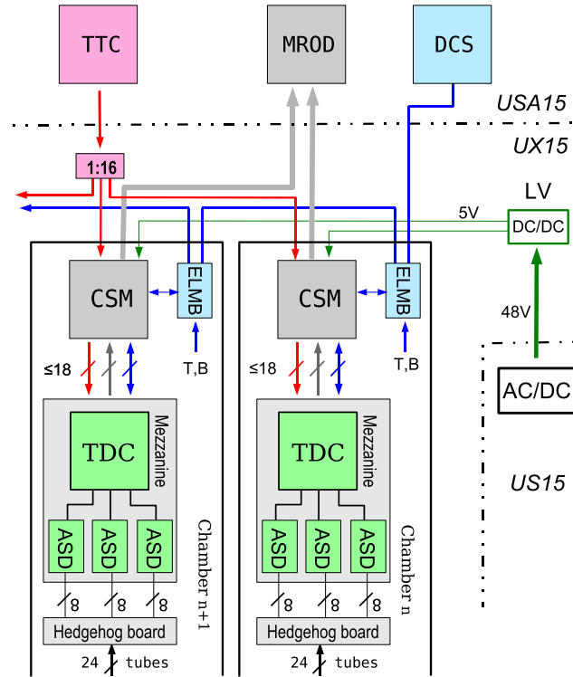
Figure 5. Schematic diagram of the MDT readout electronics. Each CSM serves up to 18 mezzanine boards depending on chamber size, each MROD up to 6 CSM's.
