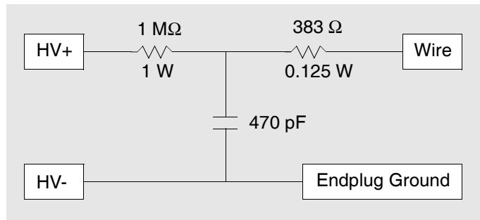
Figure 10. Schematic of one HV hedgehog channel.
