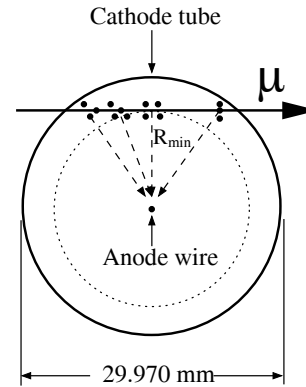
Figure 2. MDT tube cross section with a distribution of ionization clusters along a track.
