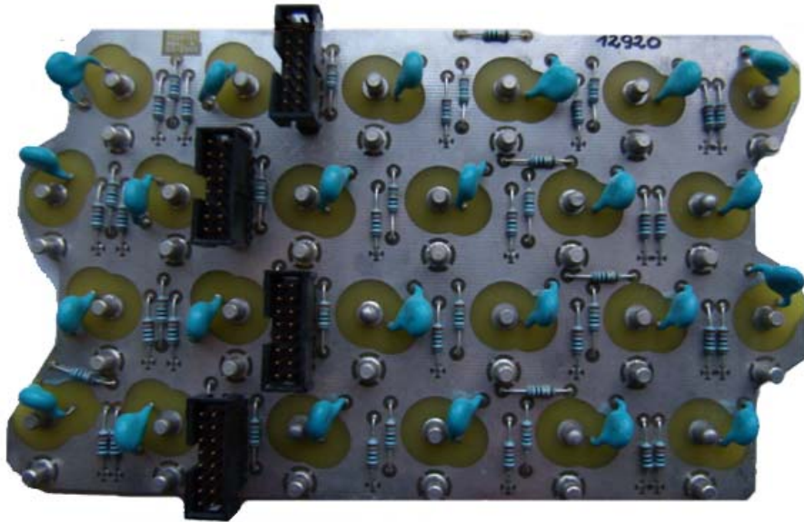
Figure 9. A signal hedgehog board for 4 tube layer chambers.
