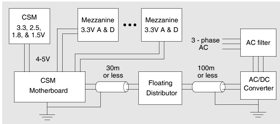
Figure 30. Low-voltage DC power distribution. Three phase AC power is filtered and transmitted to AC/DC converters that output 48 VDC. The 48 V is then transmitted to DC/DC converters called Distributors, that each provide approximately 5 V output to several chambers. At the chamber CSM a nominal value of 4 V is needed after resistive losses in the cables. From the motherboard, the unregulated but filtered 4V power plane provides input for CSM and mezzanine card regulators. The 3.3V analog and digital regulators on the mezzanine card are referenced to separate grounds. All voltages on the CSM are referenced to a common ground plane.
