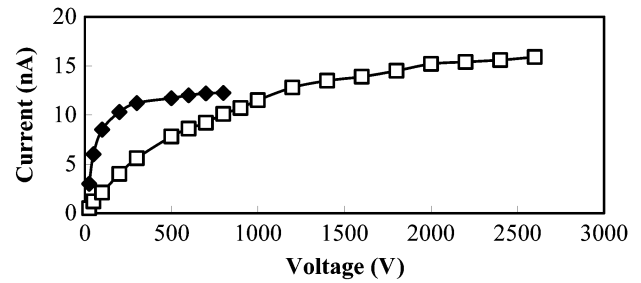
Fig. 8. Current measured by a photodiode R1259 (diamonds) and from the CsI cathode of the upper GEM (squares) in CH 4 . Note that at high voltages both currents reached plateau: I_{PD} = 12.2 nA and I_{GEM} = 15.9 nA.
