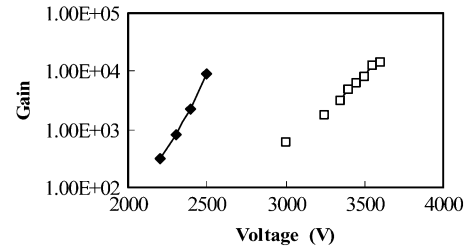
Fig. 20. Gains vs. voltage as measured in Ar (diamonds) and Ar + 20%CO 2 (squares) with the RETGEM 2.4 mm thick. As a radioactive source ^{55}\text{Fe} was used.
