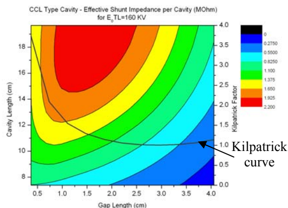
Figure 4: Effective shunt impedance (MΩ) for a CCL-type cavity.
