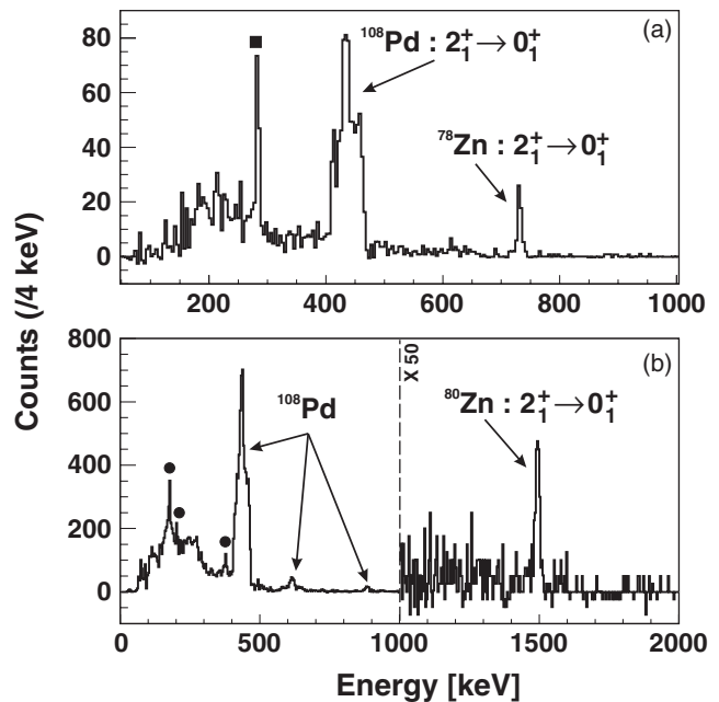
FIG. 1. Doppler corrected for the detected beam particle and random subtracted \gamma spectra during laser-ON periods, gated by detected ^{78}\text{Zn} , Ga (a) and ^{80}\text{Zn} , Ga, Rb (b) particles. The filled symbols indicate \gamma lines following Coulomb excitation of the dominant isobaric contaminants (circles = ^{80}\text{Rb} , square = ^{78}\text{Ga} ).
