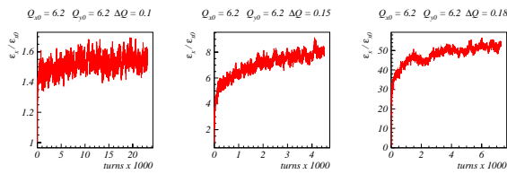
Figure 2: Emittance growth in a PS-like ring for a single constant electron lens adjusted to compensate a peak s.-c. tune shift \Delta Q^{SC} of 0.1 (left), 0.15 (center) and 0.18 (right). Head and tail particles are overcompensated, and they become transversely unstable for \Delta Q^{SC} > 0.13 .
