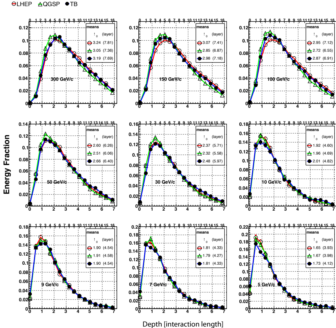
Figure 13: Longitudinal energy profile observed in HCAL in comparison to GEANT4 for beams of 300, 150, 100, 50, 30, 10, 9, 7, and 5 GeV/c pions.
