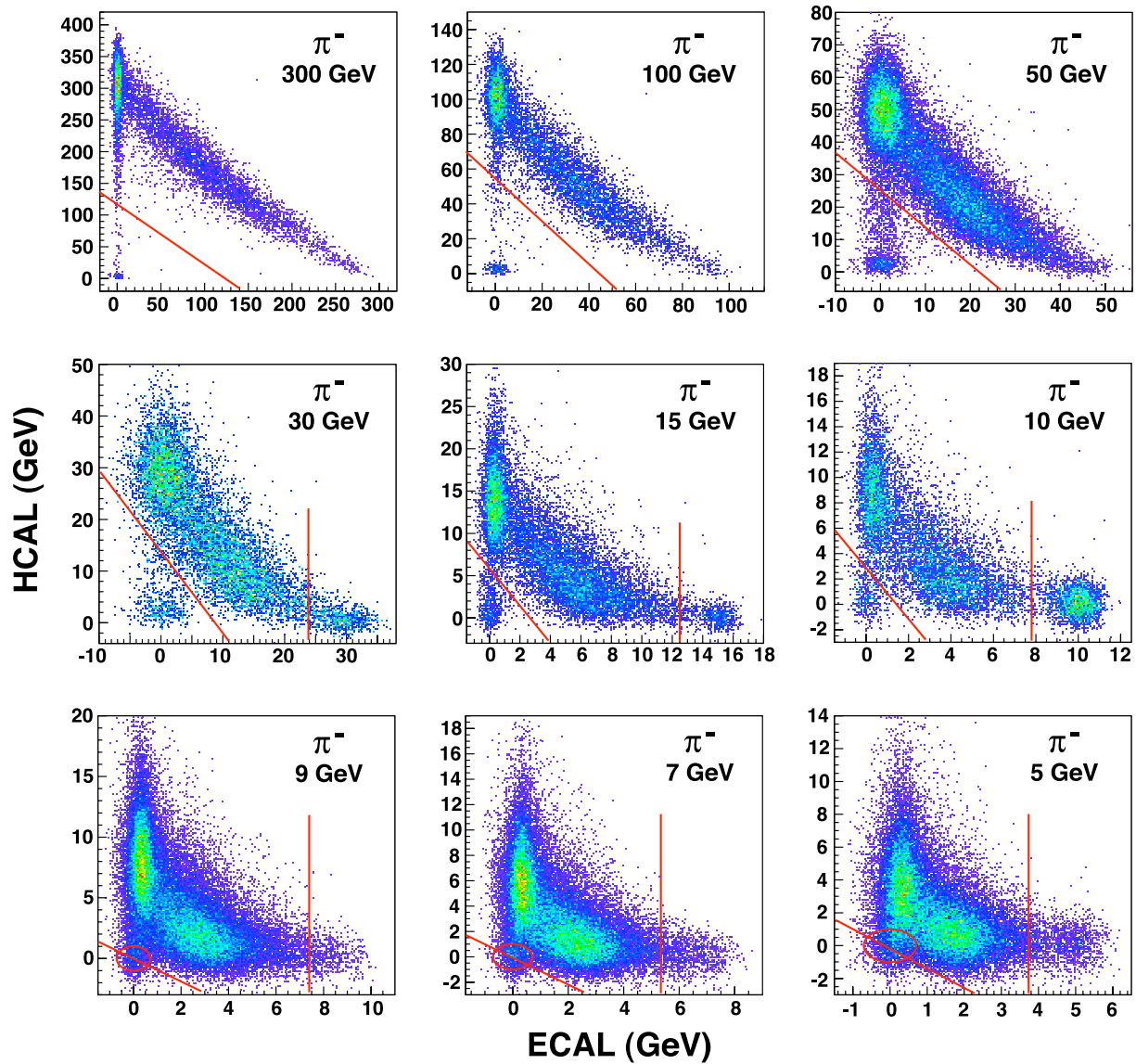
Figure 3: Energy observed in HCAL vs. energy observed in EBP for beams of 300, 100, 50, 30, 15, 10, 9, 7, and 5 GeV/ c pions. Cuts used to reject electrons (vertical lines) and muons (diagonal lines and ellipses) are indicated. A long “tail” with little EBP energy and reduced HCAL energy due to upstream interactions is also evident.
