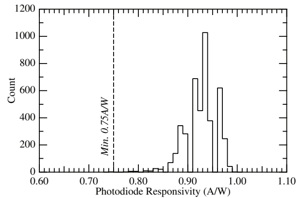
Figure 12: Showing the histogram of Photodiode Responsivity for all delivered components.
