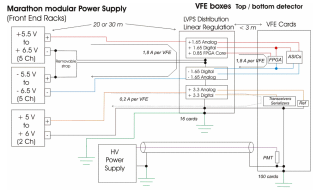
Figure 7. Power supply distribution
