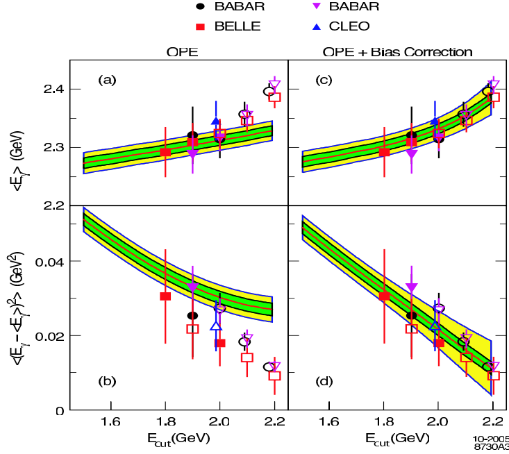
Fig. 7: The first and second moments of the photon energy in B \rightarrow \gamma X compared to OPE predictions without and with bias corrections. The inner band indicates the experimental uncertainties only; the outer bands add the theoretical ones; from Ref. [66]
