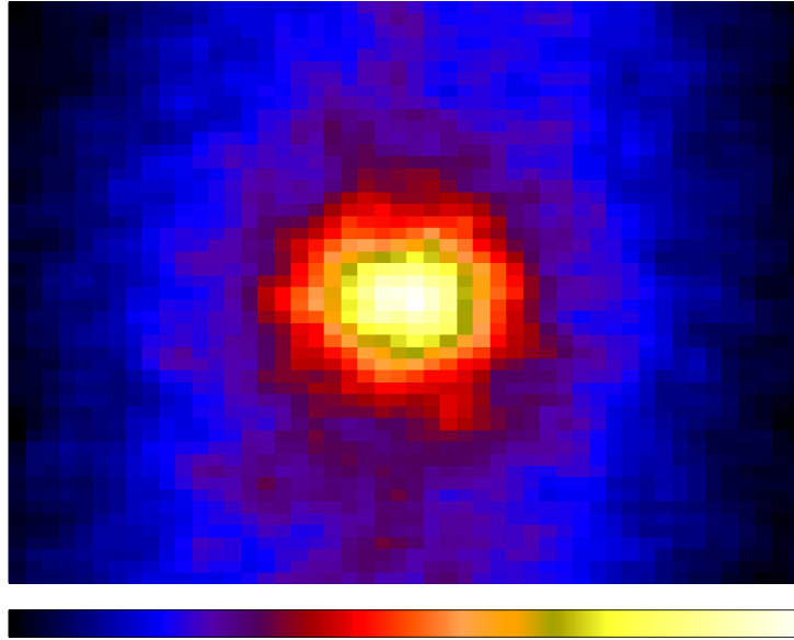
Fig. 8: The sun in the light of its neutrino emission as seen by the Super-Kamiokande detector; from Ref. [87]
