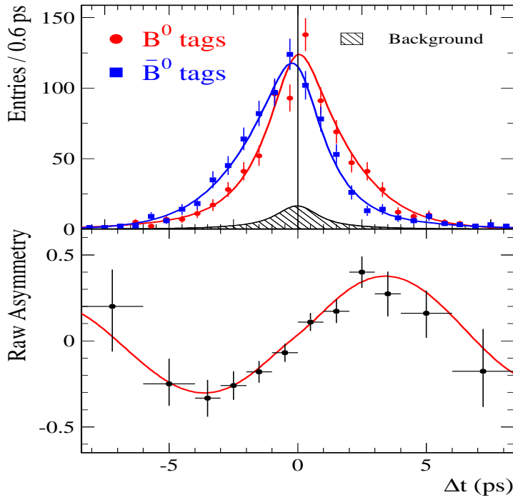
Fig. 6: The observed decay time distributions for B^0 (red) and \bar{B}^0 (blue) decays.
