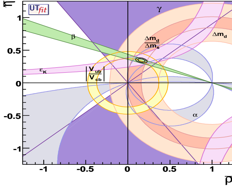
Fig. 3: The CKM Unitarity Triangle fit.
