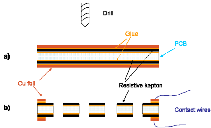
Fig. 2. Two step process in drilling holes in improved RETGEM: a) On the top of the PCP a resistive caption sheet and a Cu foil were glued; this structure was drilled through by the CNC machine b) The Cu foil was removed from the active area of the detector
