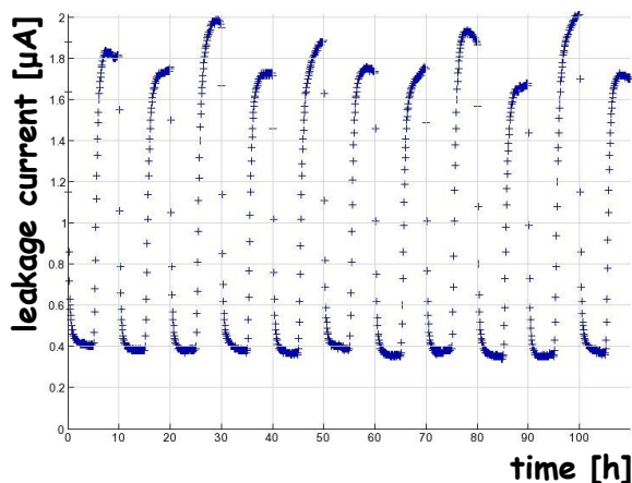
Figure 4: Leakage current as a function of time as measured during a particularly long burn-in of a Trigger-Tracker module. The periodic variation of the leakage current is due to the temperature cycling between room temperature and 5°C.
