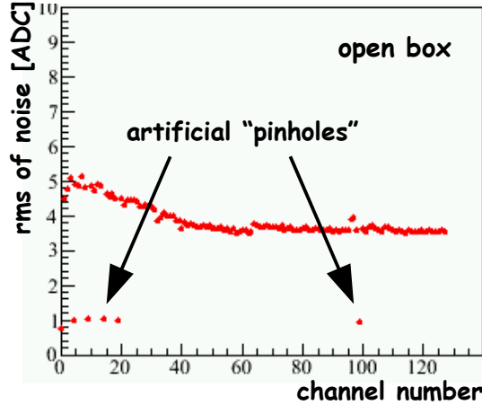
Figure 5: Root mean square of the noise distribution for each of the 128 channels on a Beetle chip, measured with an open detector box. Channels with artificially introduced “pin-holes” show up clearly due to their much reduced noise, as explained in the text.
