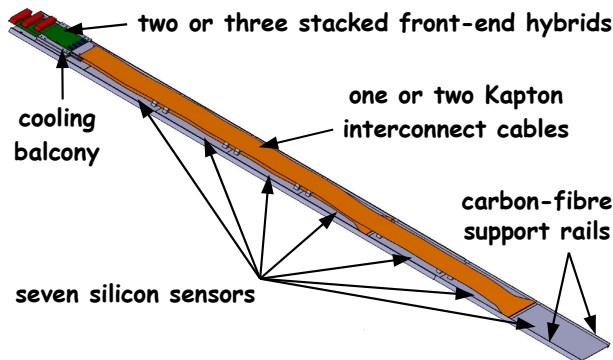
Figure 1: “4-2-1” type detector module for the Trigger Tracker.
