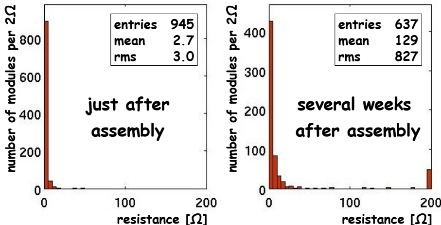
Figure 6: Distribution of the resistance across silver glue connections between bias voltage cable and sensor backplane, measured right after the module assembly (left) and a few weeks to months later (right).
