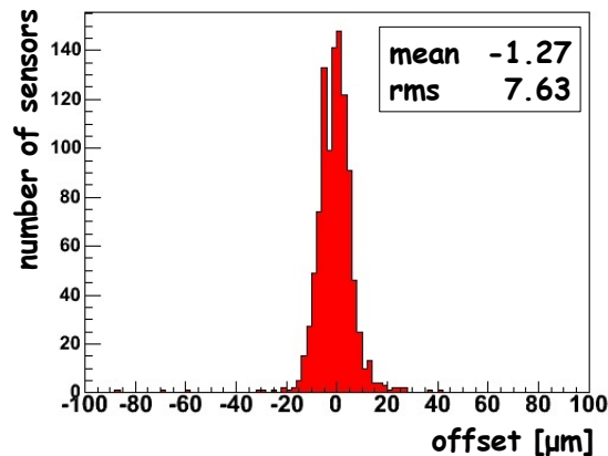
Figure 3: Distribution of the relative offsets of silicon sensors on a Trigger Tracker module.
