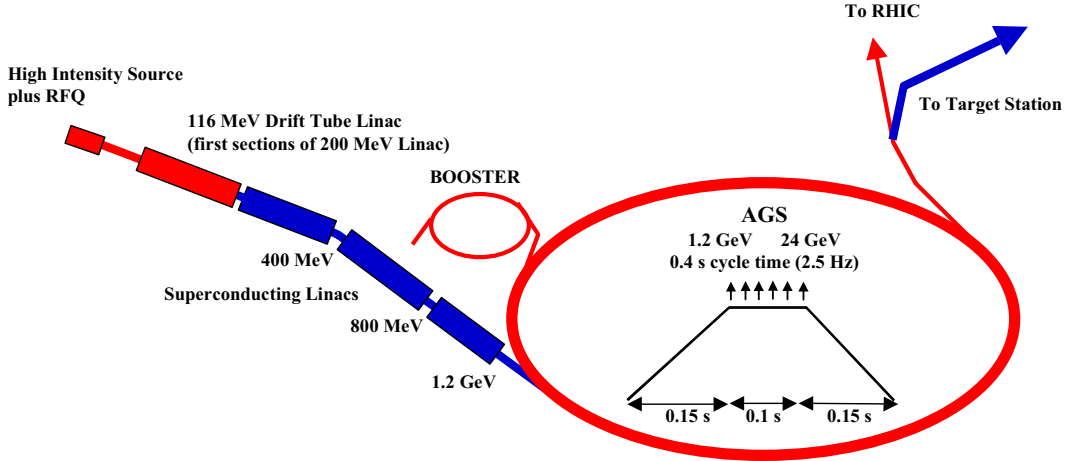
FIG. 12: (Color)AGS proton driver layout.
