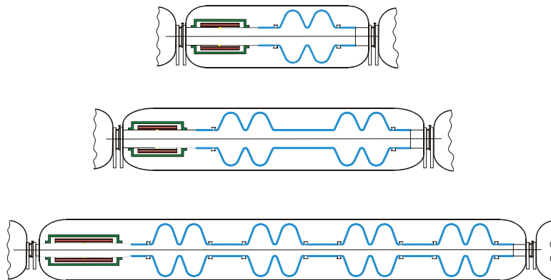
FIG. 22: (Color)Layouts of short (top), intermediate (middle) and long (bottom) cryomodules. Blue lines are the SC walls of the cavities. Solenoid coils are indicated in red.
